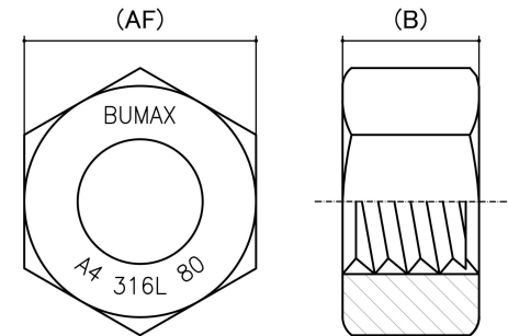
Cad Drawings shown for graphic representation only.*
